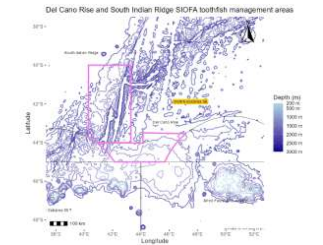
Figure B: Boundaries of the Del Cano Rise and the South Indian Ridge -areas (2024).
