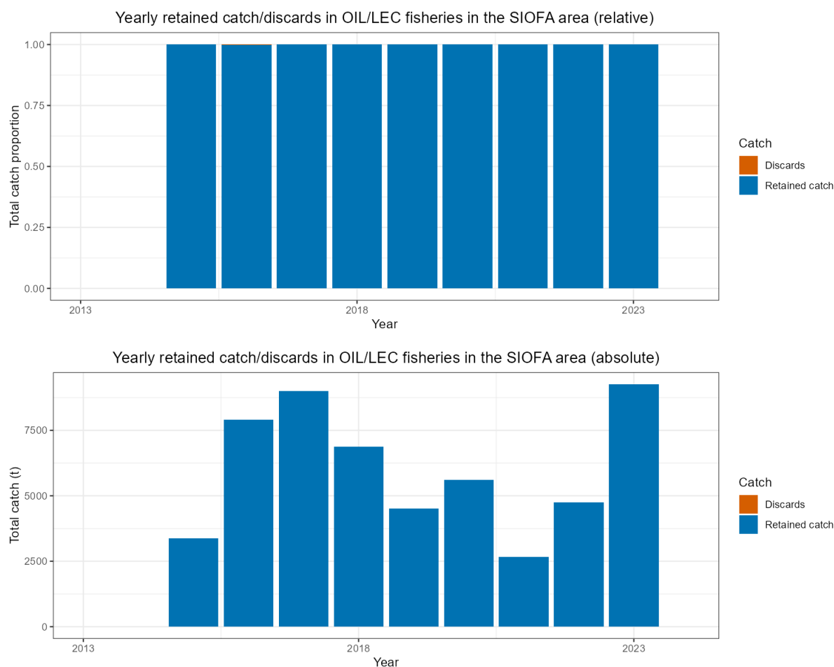
Figure 109a and b – Total retained and discarded catch in SIOFA fisheries that targeted oilfish, shown as relative values (upper panel, a) and absolute values (lower panel, b) (source: SIOFA AggregatedCatchEffort and HBHCatchEffort databases 2014–2023). Catches reported without location information are not included.
