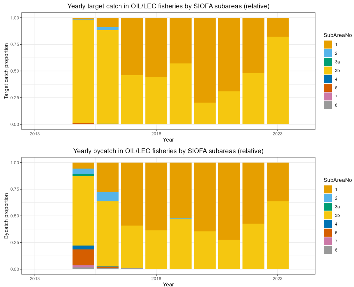
Figure 98a and b – Distribution of target catch (a) and bycatch (b) in fisheries targeting oilfish in different SIOFA Subareas (source: SIOFA AggregatedCatchEffort and HBHCatchEffort databases 2014–2023). Catches reported without location information are not included.
