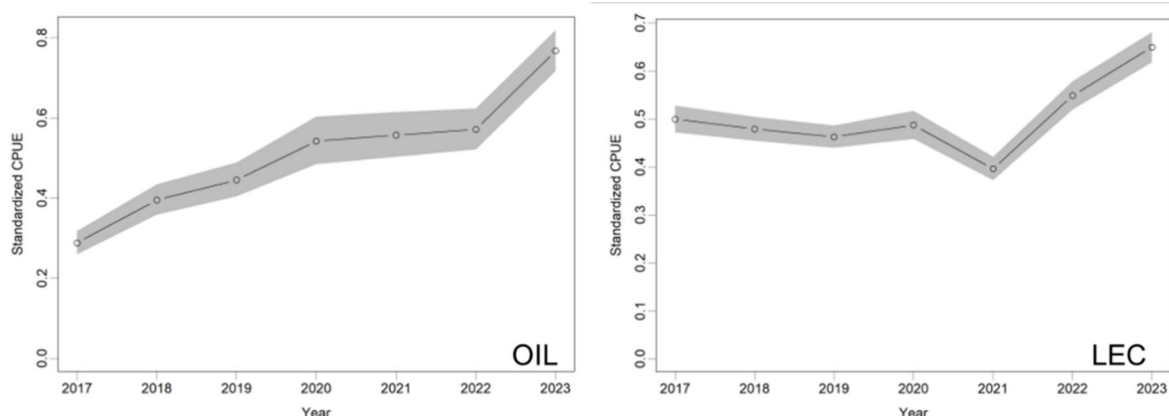
Figure 5 - Standardized CPUE index of oilfish and escolar in oilfish fishery. Shaded areas illustrate the 95% confidence intervals. Source: paper SC-10-75 (restricted paper)
