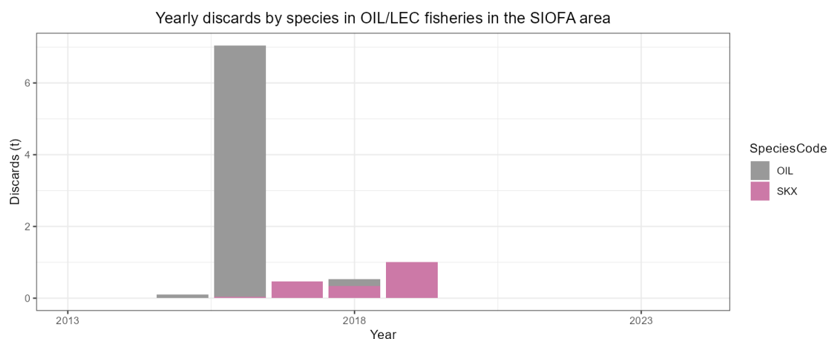
Figure 110 – Reported discards of fish species in fisheries targeting oilfish (source: SIOFA AggregatedCatchEffort and HBHCatchEffort databases 2014–2023).
