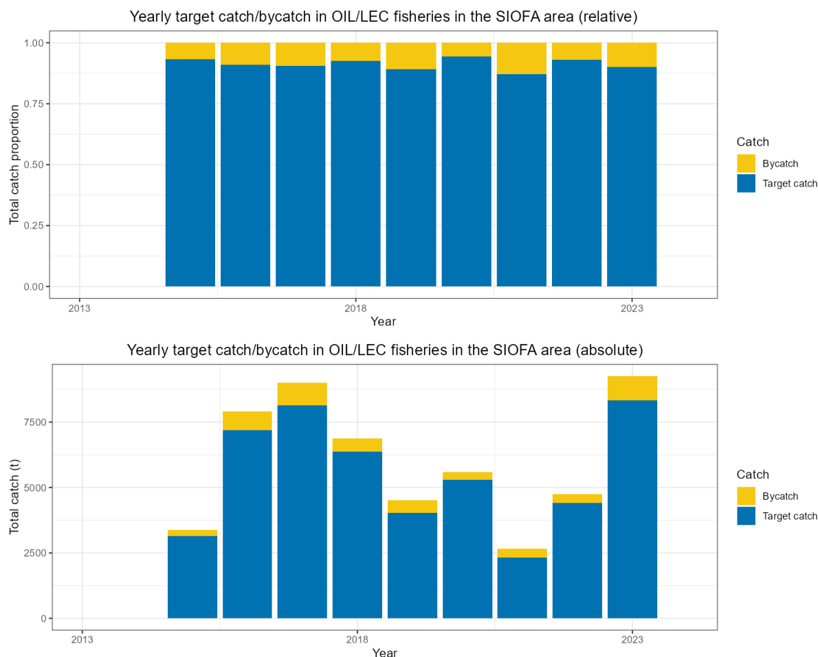
Figure 65a and b – Total catch of oilfish and other bycatch species in SIOFA fisheries that targeted oilfish, shown as relative values (upper panel, a) and absolute values (lower panel, b) (source: SIOFA AggregatedCatchEffort and HBHCatchEffort databases 2014–2023).
